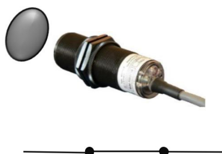
检测到目标 常开触点闭合 Closes when target is seen
