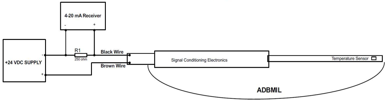
Figure 2- Typical Connection
